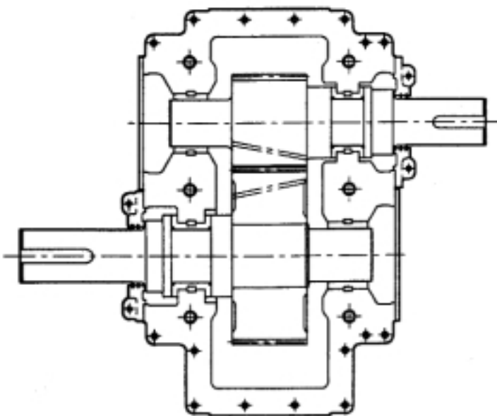
SINGLE HELICAL GEARING WITH TAPER LAND THRUST BEARINGS
